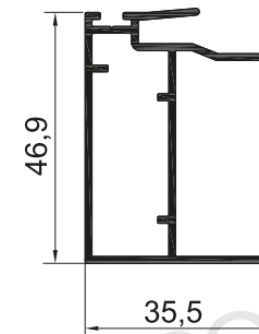
Cruce ventana Ref. 44.2370
