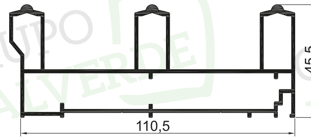
Marco 3 carriles Ref. 44.1500
