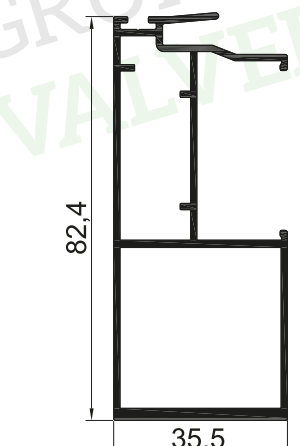
Cruce balconera Ref. 44.2371
