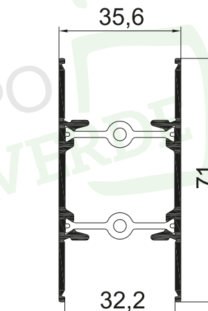
Travesaño hoja Ref. 68.2470
