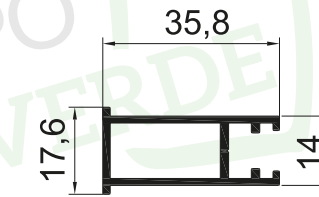
Acople 3/4 hojas Ref. 68.6500
